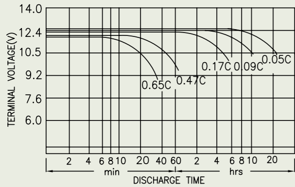
DISCHARGE CURVES (30°C,86°F)
